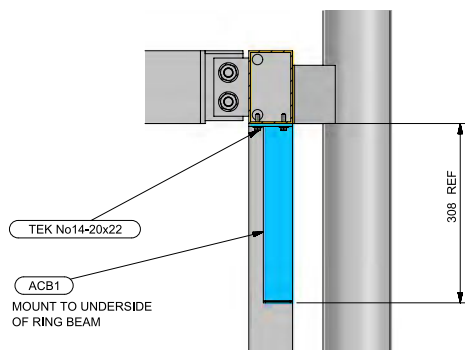
SECTION B-B SCALE 1:5
