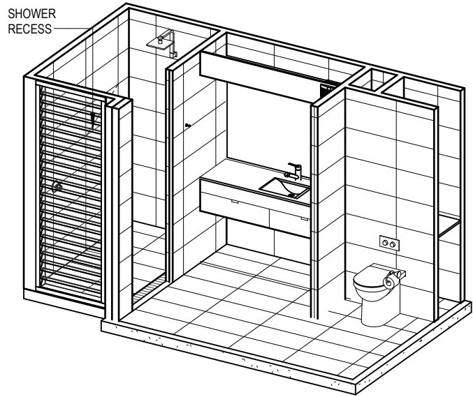
FRONT AXO
