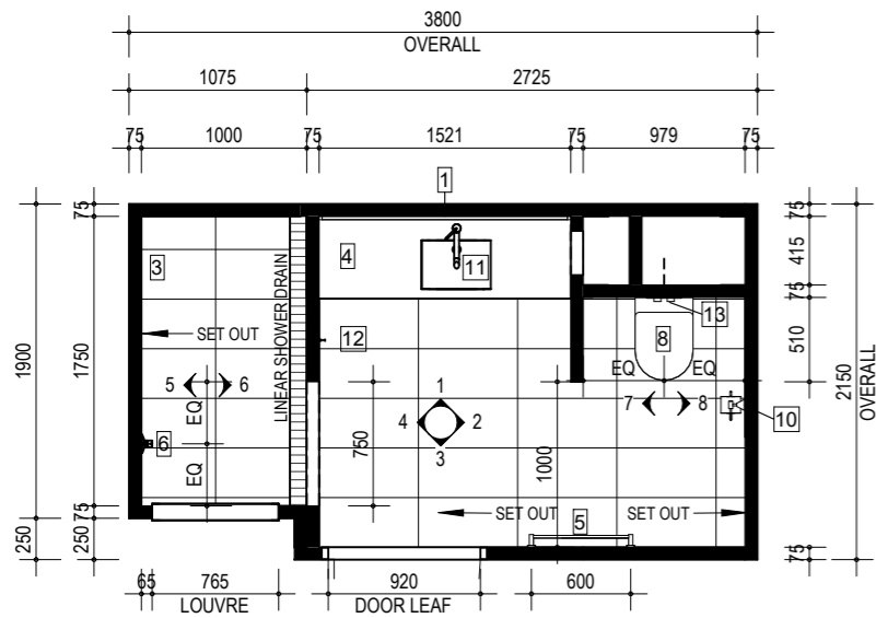
FLOOR PLAN
