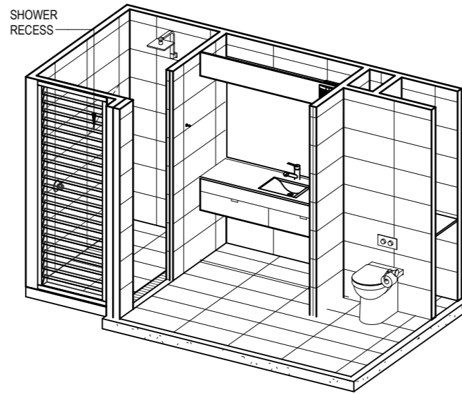
FRONT AXO
